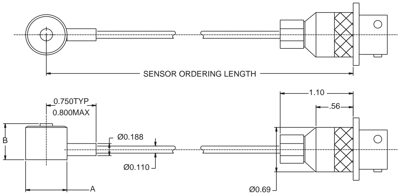
BUTTON STYLE SENSOR DIMENSIONS
